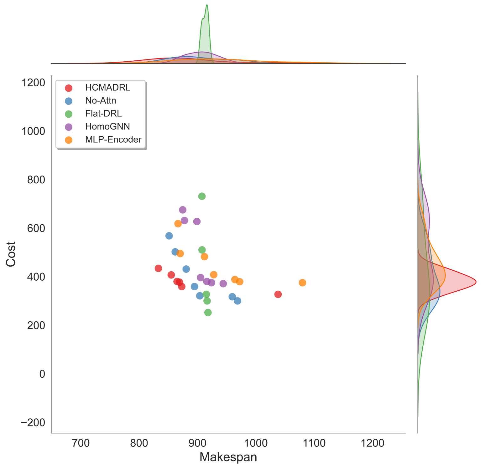
Pareto Front: Makespan and Cost (M8_A10_R6_J3)
